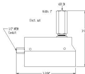
MPE-BZE
