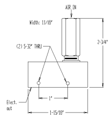
MPE-BZ
