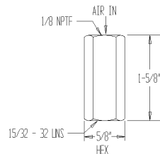
MPE-B (Actuator Head)
